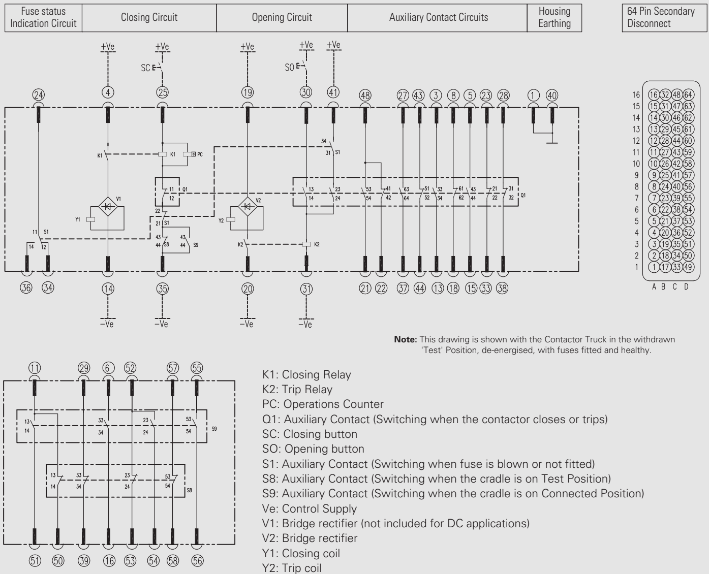
Mechanical latching Wiring Diagram of W-SLC withdrawable vacuum contactor-fuse combination units
