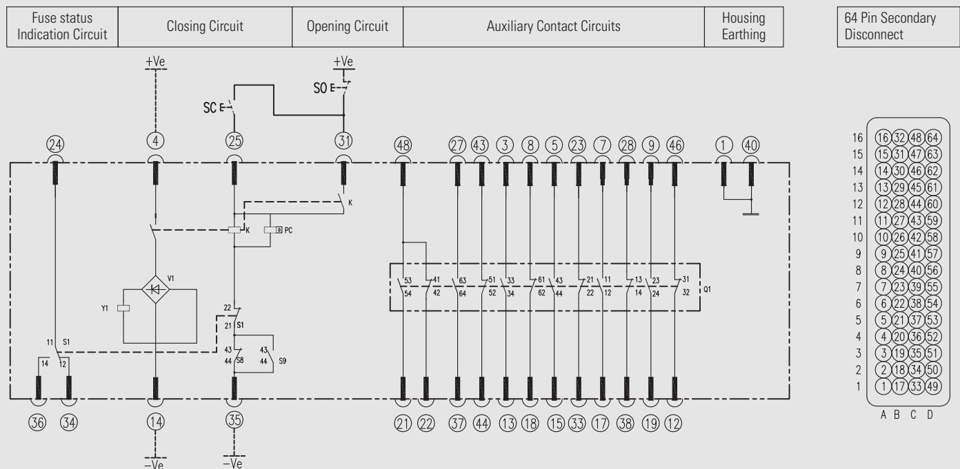
Electrical Operation Wiring Diagram of W-SLC withdrawable vacuum contactor-fuse combination units
